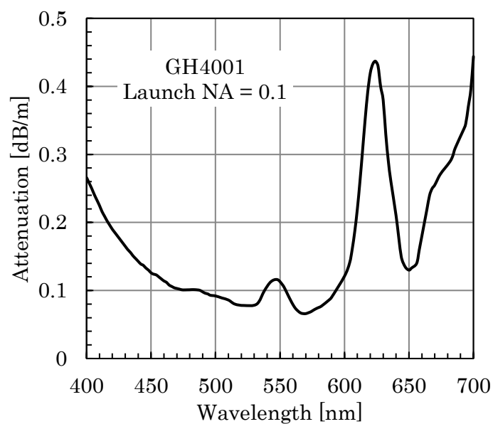
Fig. 1-1 The attenuation spectrum of the ESKA PREMIER ® cable GH-4001
