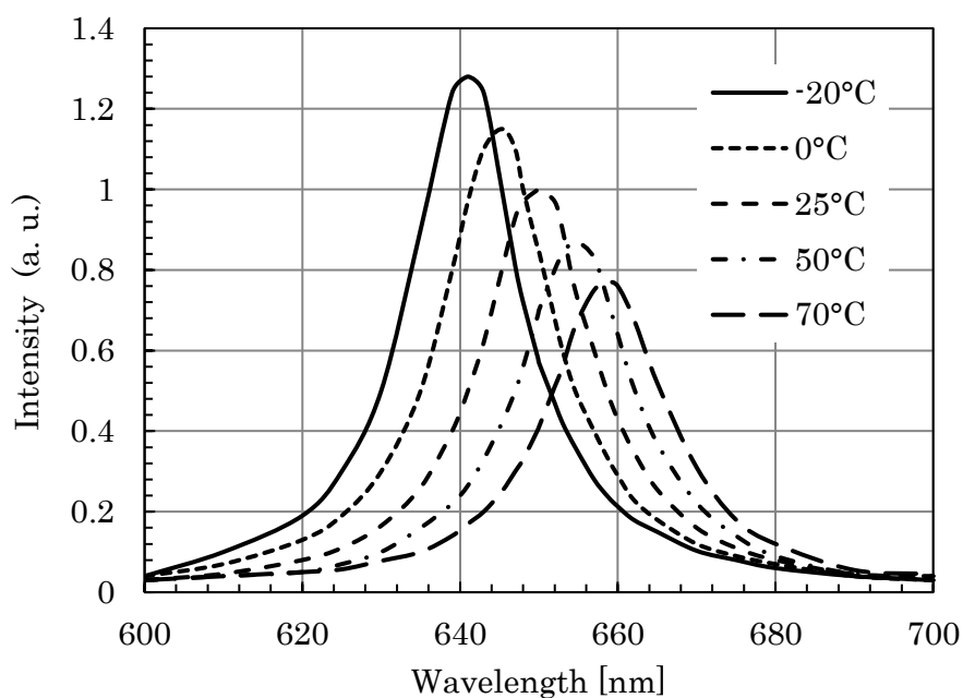
Fig. 2-4 The temperature dependences of the LED spectra
