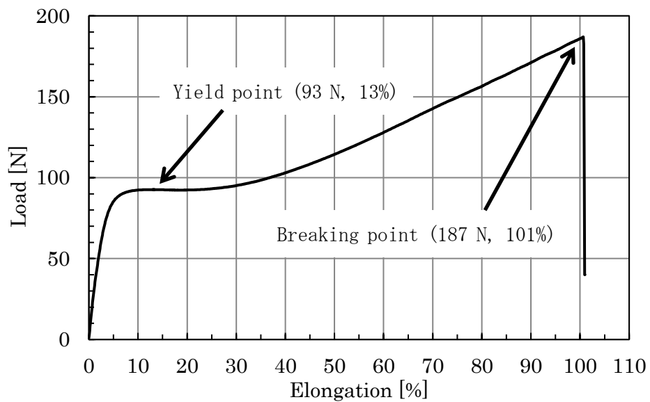
Fig. 4-3 The tensile property of the ESKA PREMIER ® cable GH-4001
