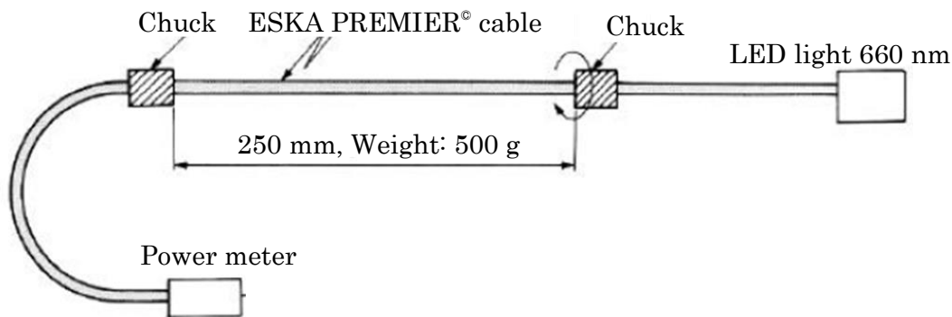
Fig. 4-6-b The schematic of the twisting test
