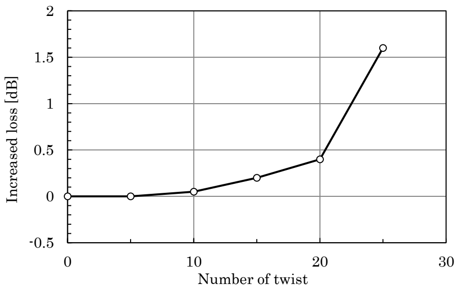
Fig. 4-6-a The increased loss of the ESKA PREMIER® cable GH-4001 in the twisting tests
